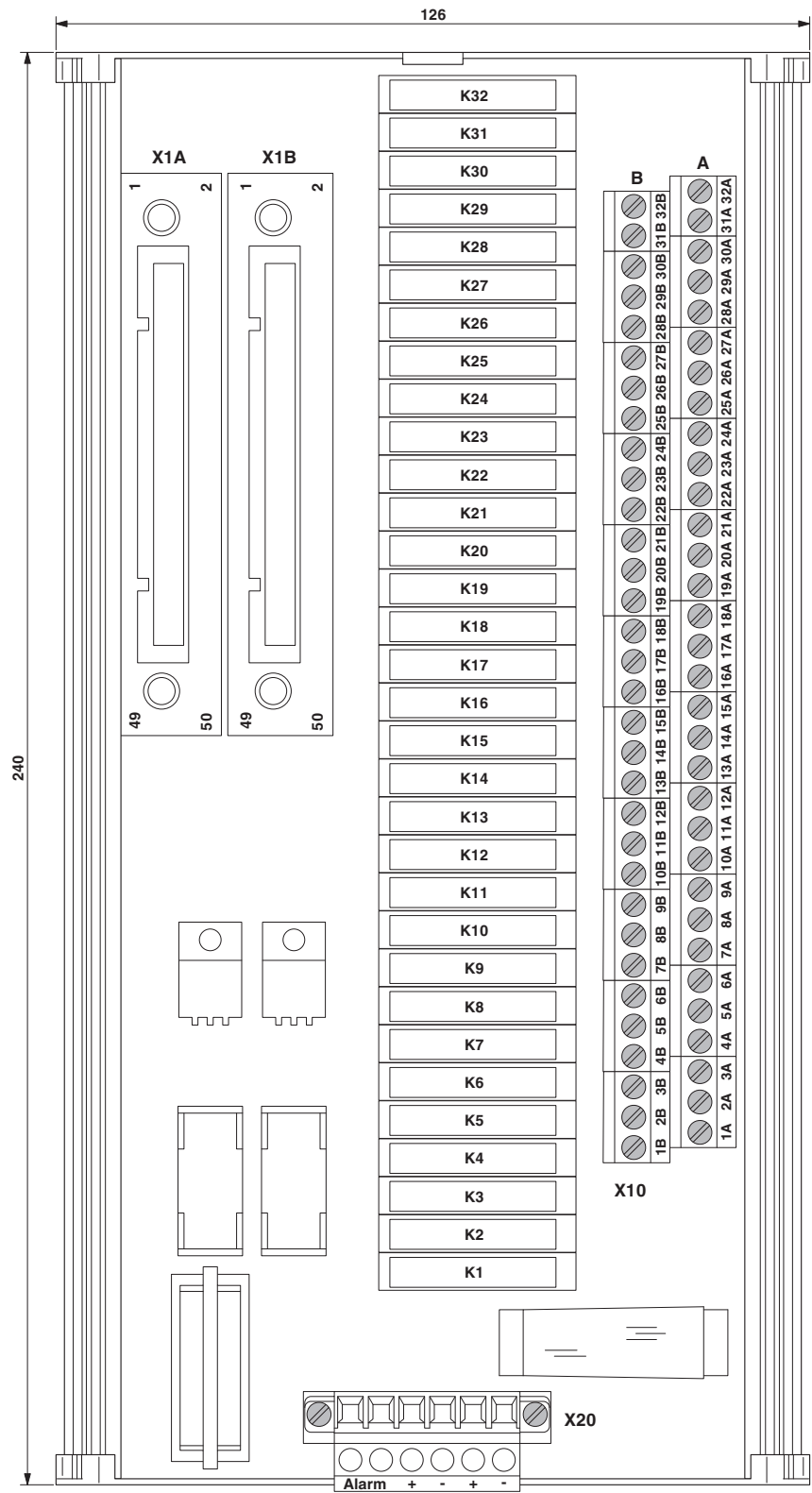
Dimensional drawing
