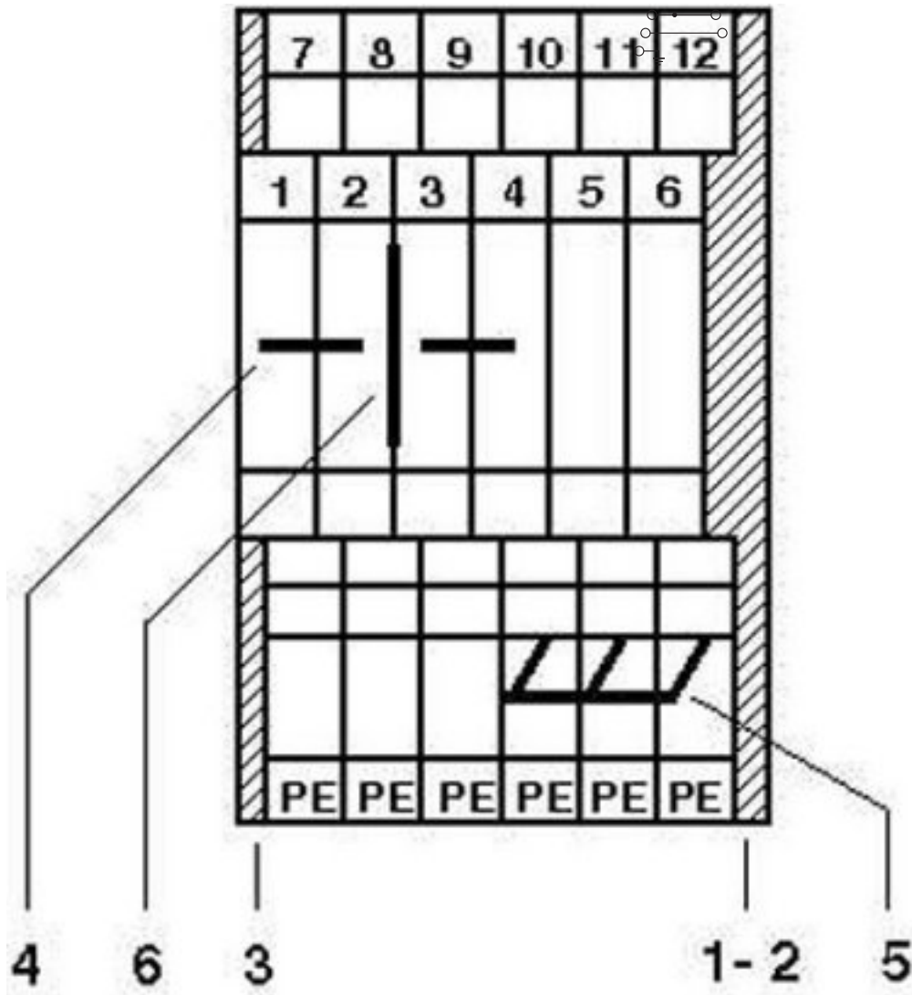
Circuit diagram
