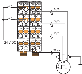
Connection diagram
