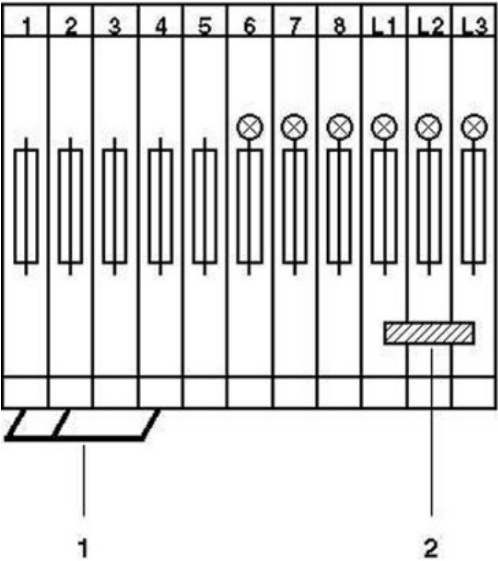
Circuit diagram
