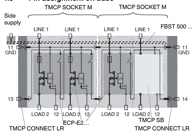
Figure 6 Connection diagram
