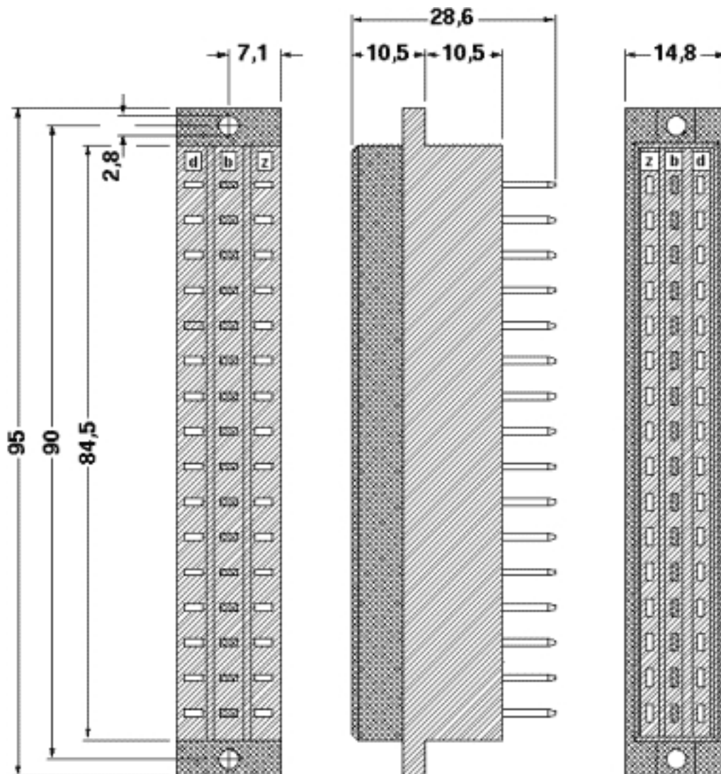
Dimensioned drawing
