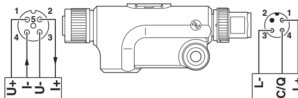
Figure 5 Connection example
