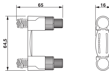
Dimensioned drawing
