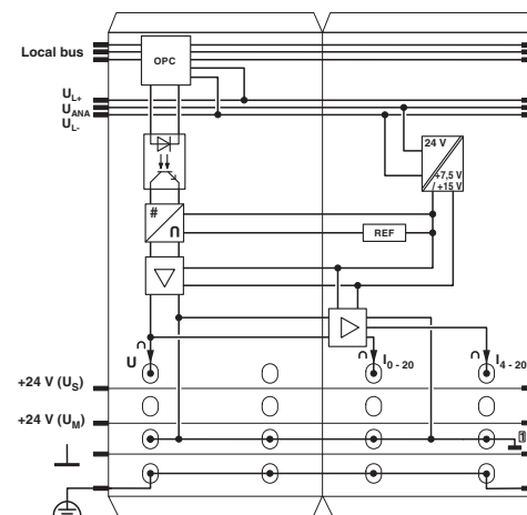
Block diagram
