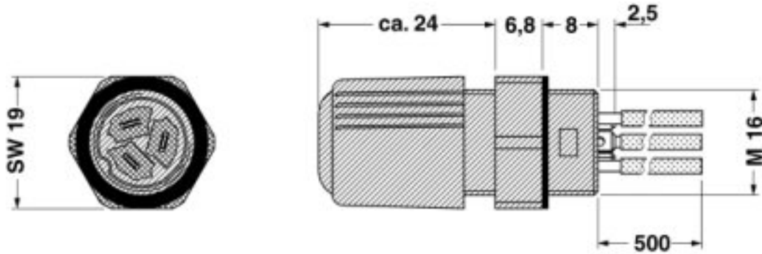
Dimensioned drawing
