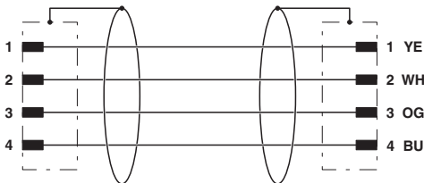
Contact assignment of M8 plugs
