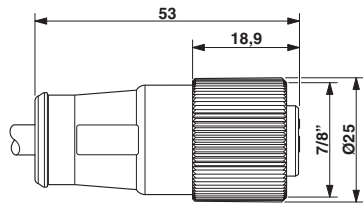
7/8"-16UNF socket, straight
