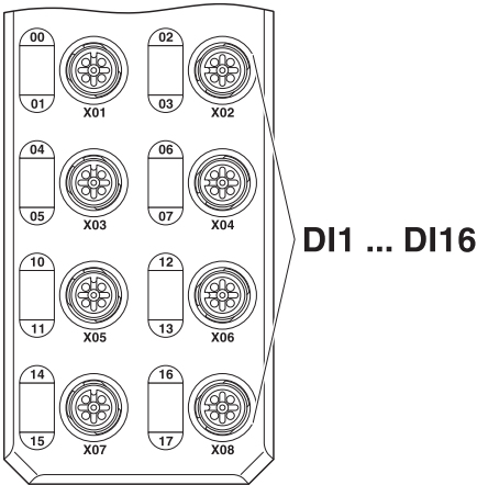
Figure 5 Input connections
