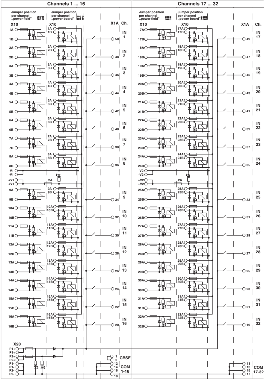
Circuit diagram
