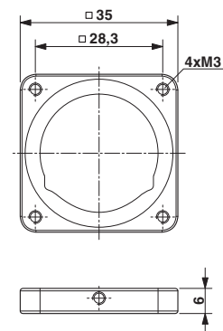
Dimensioned drawing
