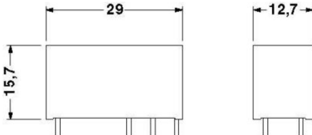
Dimensioned drawing
