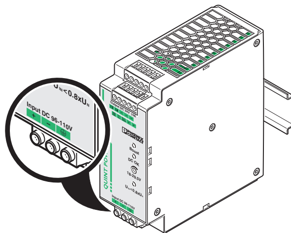
Figure 6 Input
