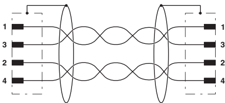
Contact assignment of the M12 plugs
