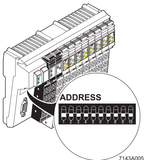
Figure 4 DIP switches of the module
