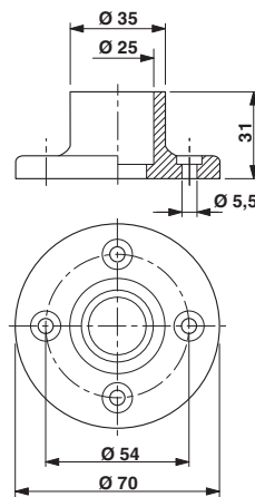
Dimensioned drawing
