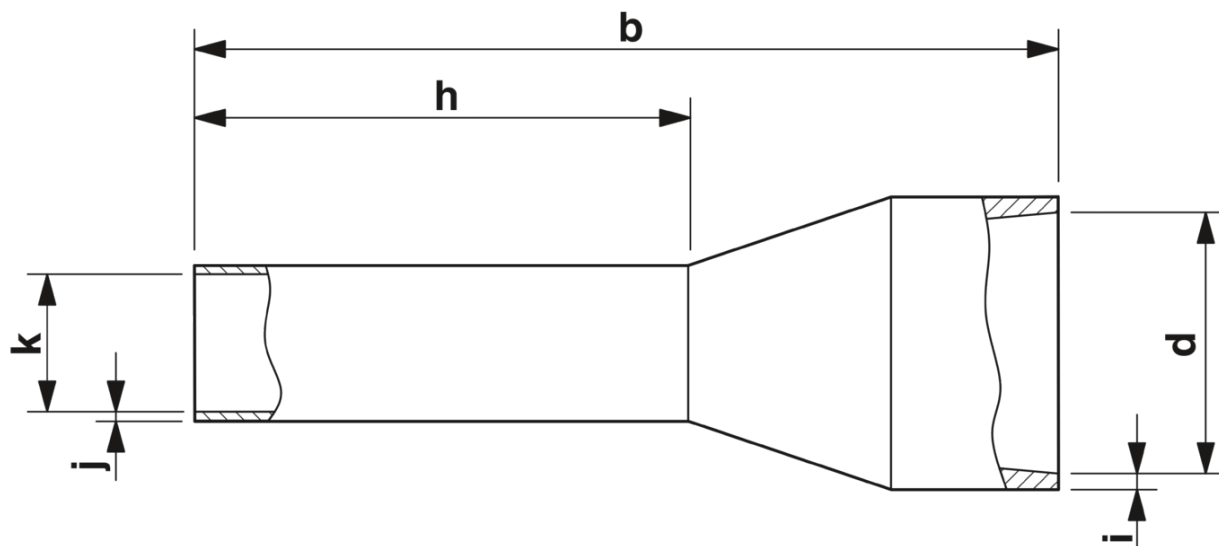
Dimensional drawing
