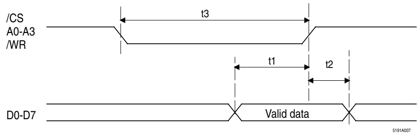
Figure 3-1 MFP interface timing, write access
