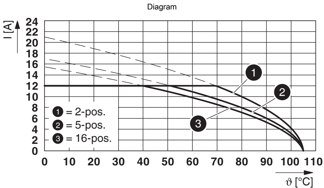
Type: FKCVW 2,5/...-STF-5,08 with MSTBV 2,5/...-GF-5,08
