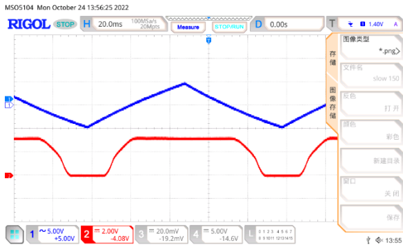
V_{IN} slow on/off 150mA, V_{OUT}=3.3V
