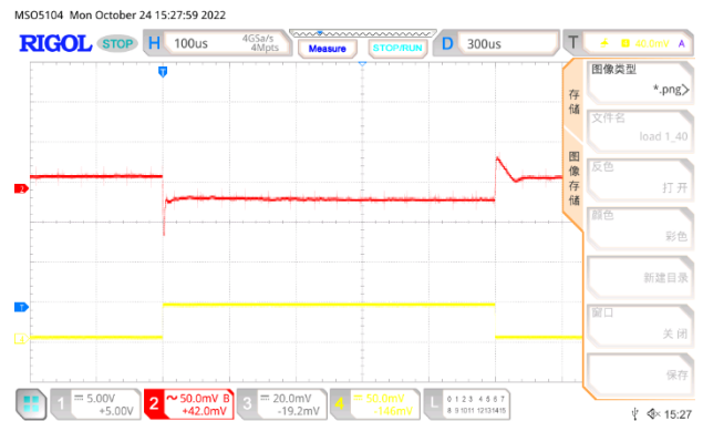
Load transient V_{OUT}=5.0V , I_{OUT}=1mA-40mA
