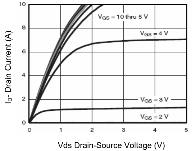
Figure 2 Output Characteristics
