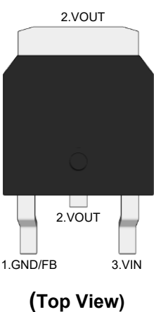
TO-252
