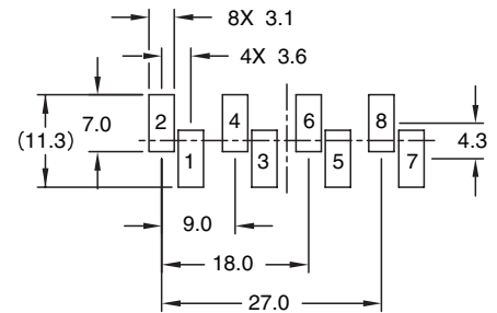
SUGGESTED LAND PATTERN TOLERANCE ON PADS = ± 0.05
