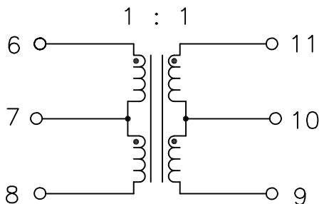
SCHMATIC
