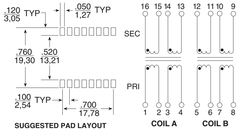
SUGGESTED PAD LAYOUT
