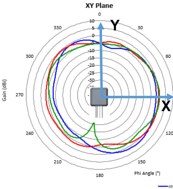
Gain Plots LTE 1
