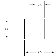
SUGGEST LAND PATTERN
