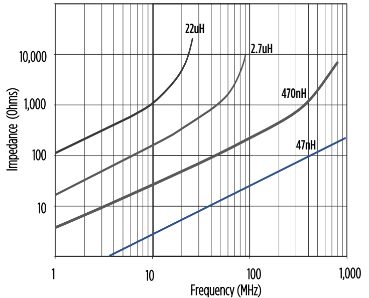
Typical Impedance vs Frequency
