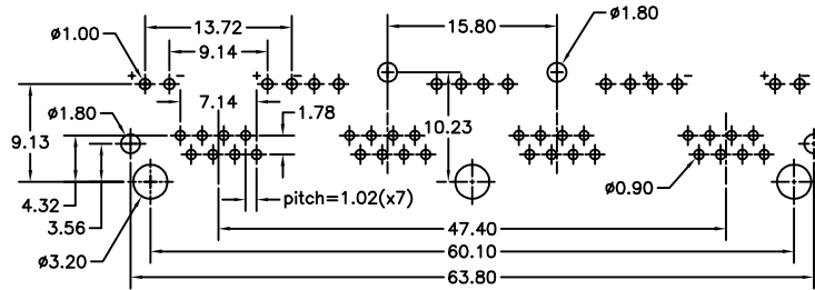
PC Board Layout T=1.6mm. Component Side Shown Tolerance±0.05mm
