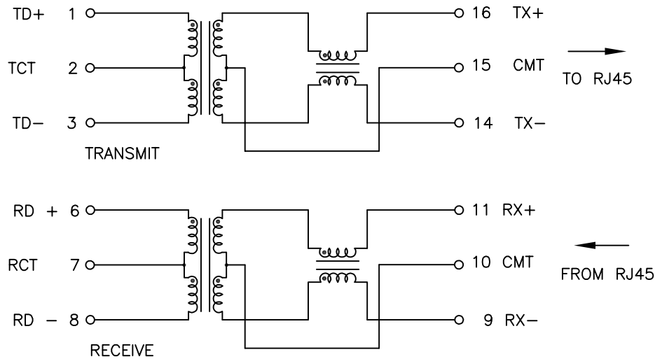
SCHMATIC
