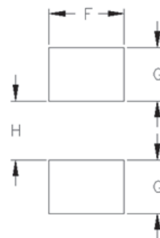
SUGGESTED PAD LAYOUT
