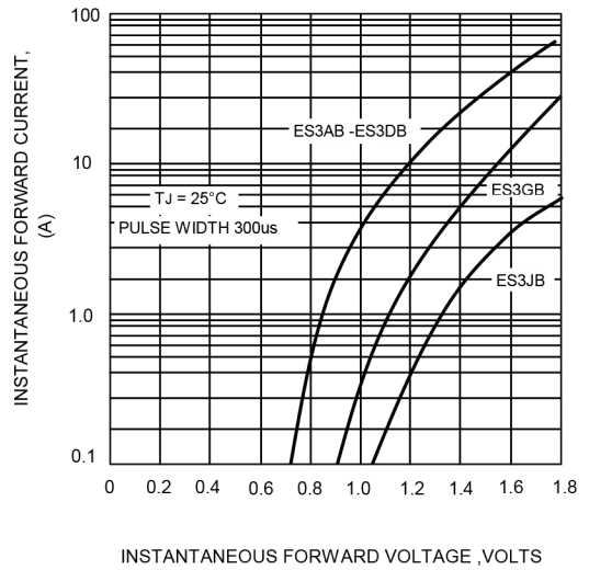
FIG.4-TYPICAL FORWARD CHARACTERISTICS
