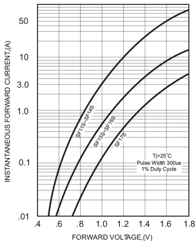
FIG.3-TYPICAL FORWARD CHARACTERISTICS
