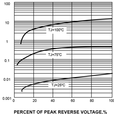
FIG. 4-TYPICAL REVERSE CHARACTERISTICS
