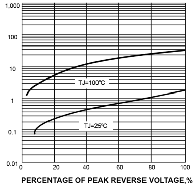
FIG. 4-TYPICAL REVERSE CHARACTERISTICS
