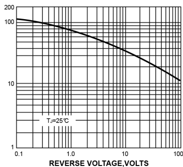
FIG. 5-TYPICAL JUNCTION CAPACITANCE
