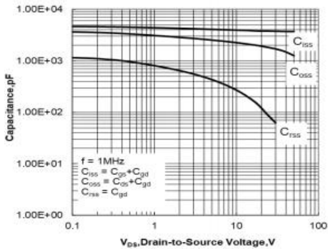
Figure 5. Capacitance Characteristics
