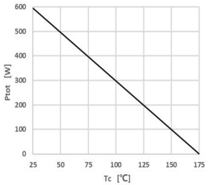
Figure 4 Power Dissipation
