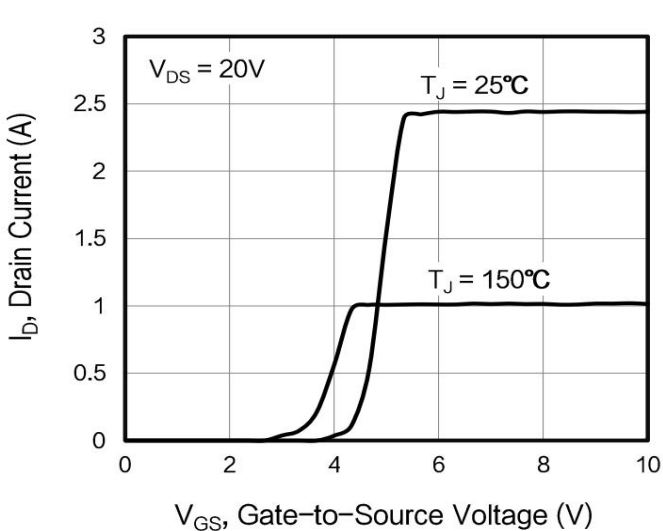
Figure 5. Transfer Characteristics
