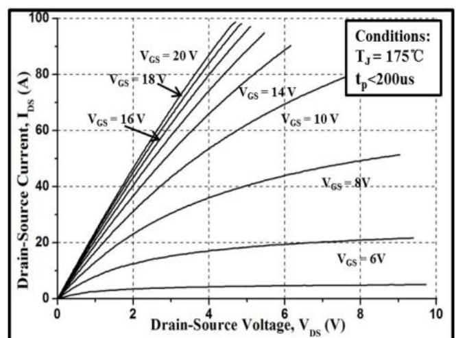
Figure 2. Typical Output Characteristics T J =175°C
