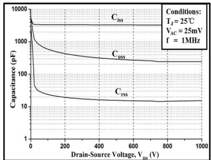
Figure 14. Capacitances vs. Drain-Source Voltage
