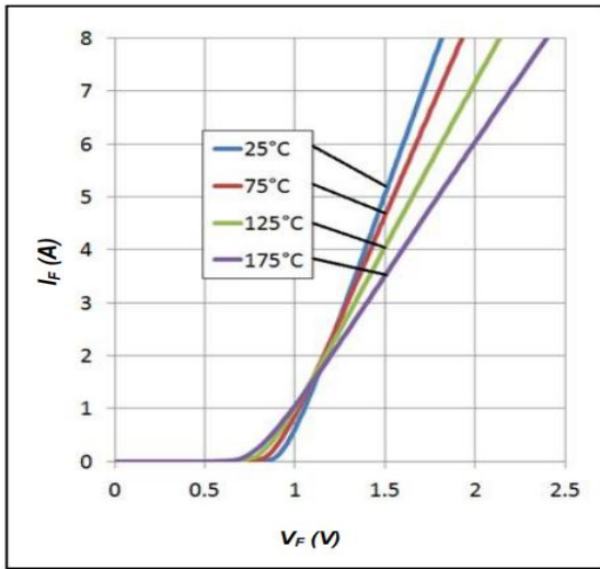
Figure 1. Forward Characteristics
