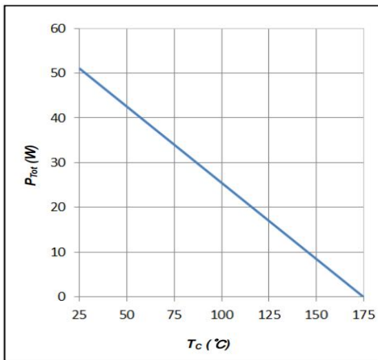
Figure 3. Power Derating
