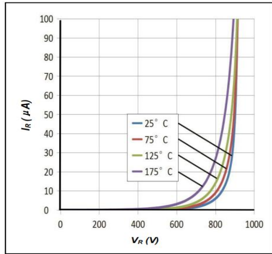
Figure 2. Reverse Characteristics
