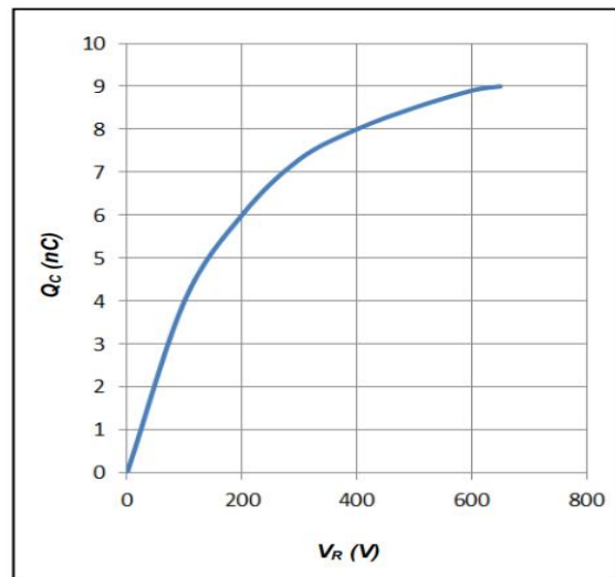
Figure 4. Total Capacitive Charge vs. Reverse Voltage
