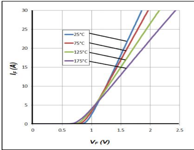
Figure 1. Forward Characteristics
