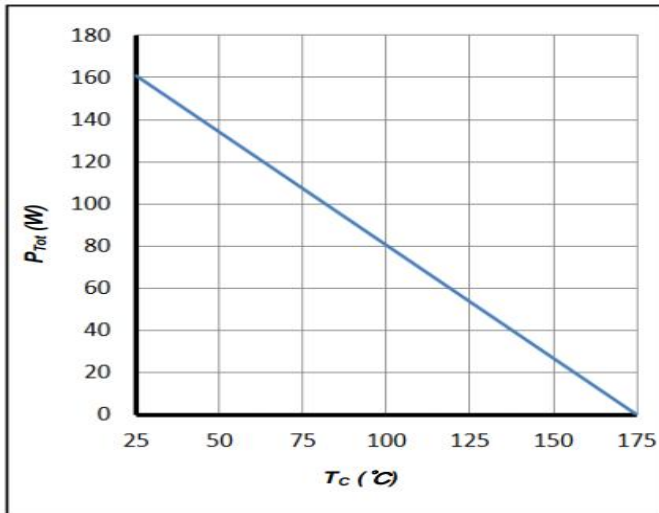
Figure 3. Power Derating
