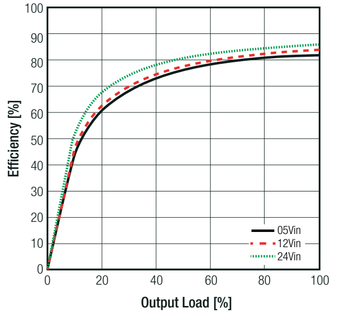
RxxP21509D Series
