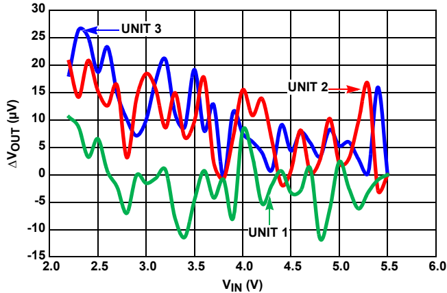
FIGURE 22. LINE REGULATION, THREE UNITS
