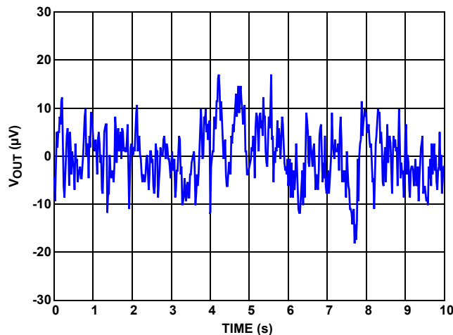
FIGURE 53. V_{OUT} vs NOISE, 0.1Hz TO 10Hz
