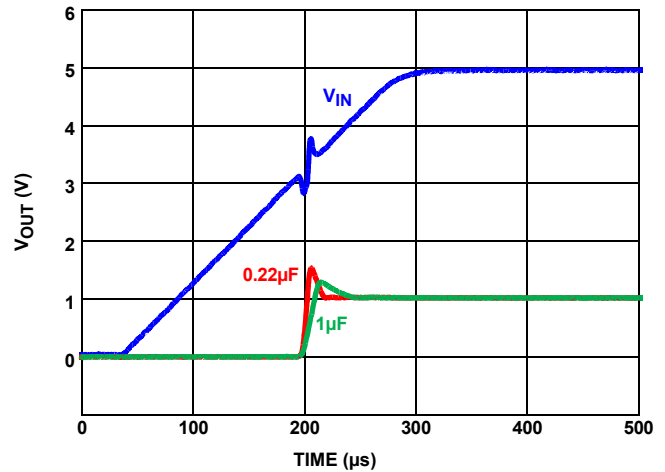
FIGURE 12. TURN-ON TIME
