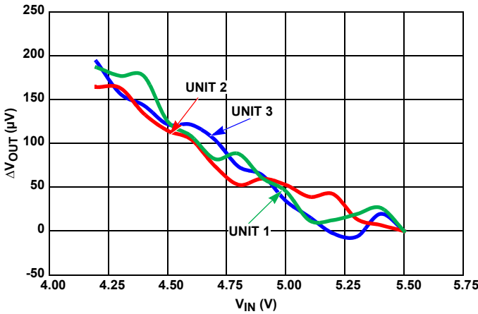
FIGURE 124. LINE REGULATION, THREE UNITS
