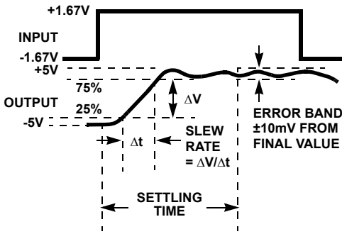
FIGURE 1. SLEW RATE AND SETTLING TIME
