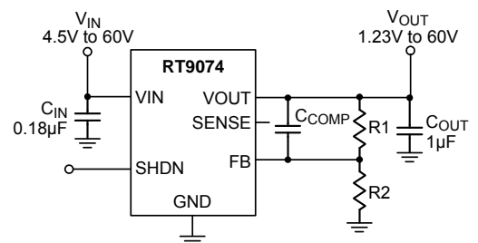
RT9074 (Adjustable Up to 60V Output)
