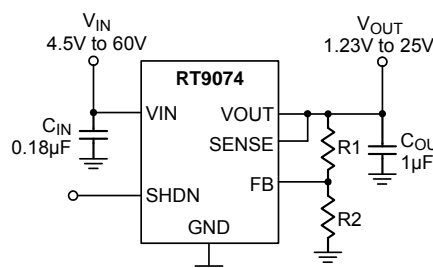
RT9074 (Adjustable Up to 25V Output)
