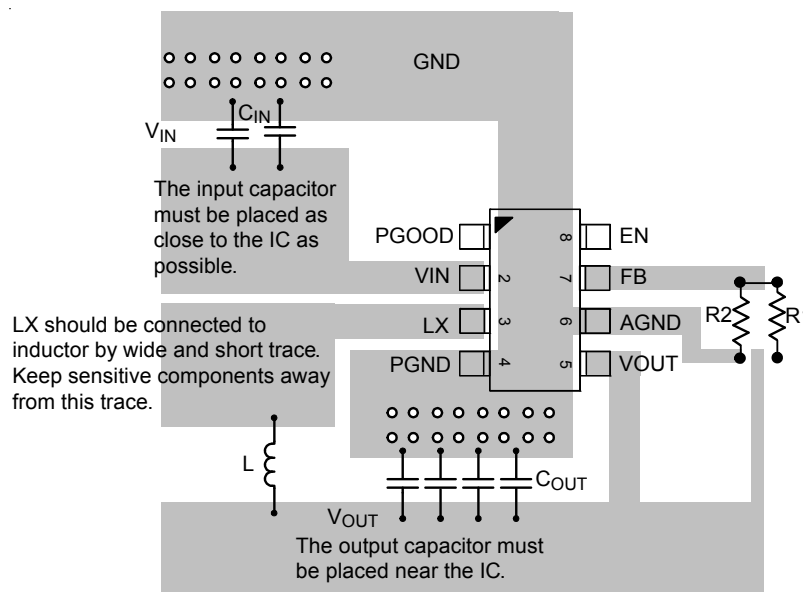
Figure 6. PCB Layout Guide
